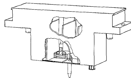
Fig. 1—Four-stage filter.
